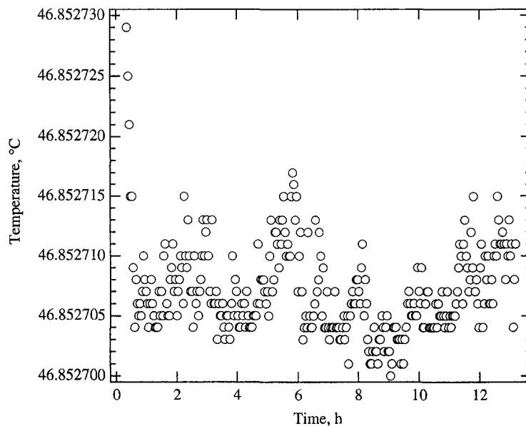
Fig. 2. The resulting cell temperature after a 1-mK temperature step using our thermostat. The temperature varied less than \pm 10 \mu\text{K} , with a standard deviation of 3.3 \mu\text{K} over a period of 12 h.
