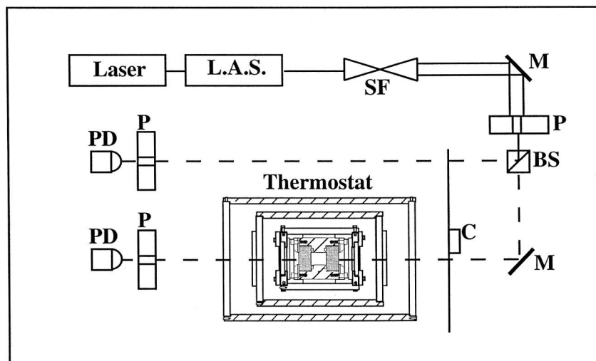
Fig. 3. Optical schematic. The laser beam passes through a laser amplitude stabilizer (L.A.S.) before passing through a spatial filter/beam expander (SF) and then striking the beamsplitter (BS). Each beam is chopped at a different frequency. The photodiodes (PD) detect the light and provide a signal to lock-in amplifiers whose reference frequencies are locked to the chopper C.
