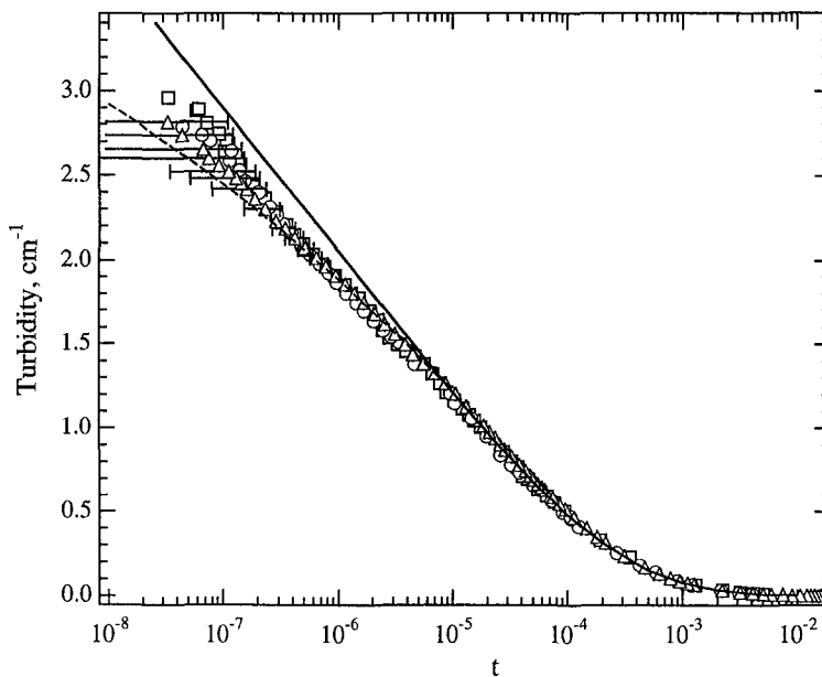
Fig. 1. Theory and preliminary data for the turbidity \tau of methanol-cyclohexane. The upper (solid) line is from Eq. (1), where the critical exponent \eta = 0 ; the bottom (dashed) line is from Eq. (2) when \eta = 0.033 . Both curves use the same parameters and constants, with the constraint that the scaling relation \gamma = \nu(2 - \eta) holds. An effect due to \eta can be detected only close to the critical point [small reduced temperature, t = (T - T_c)/T_c ]. Three experimental runs are shown—Run 1 (squares), Run 2 (circles), and Run 3 (triangles)—with representative error bars on Run 3. The error in the turbidity is smaller than the symbol size in this plot.
